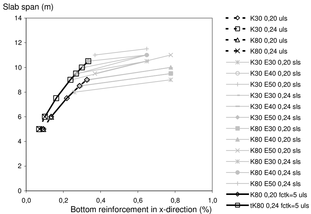
Diagram 3: Slab type 4 The same as Diagram 2 but consideration taken to punching
