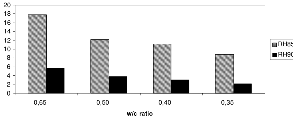
Figure 4.10 Estimated effects of various w/c ratios on the concrete drying time for Climate 3. Constant type of formwork (permanent concrete elements, “Filigran”) and slab thickness (0,20 m). No silica fume.
