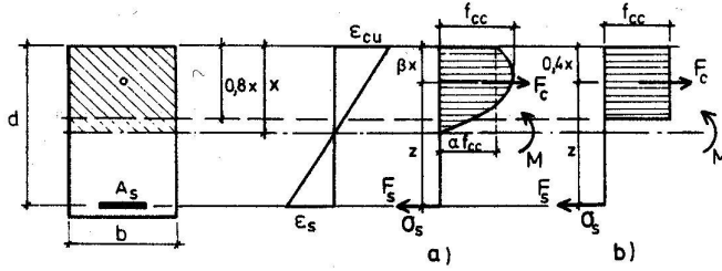
Figure 1: Stress distribution according to BHK 3.6:43, figure 3.6:12b, (a) real distribution of compressive stress, (b) simplified distribution
