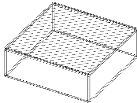
Figure 3.3 Slab type 2, single two-way reinforced slab.
