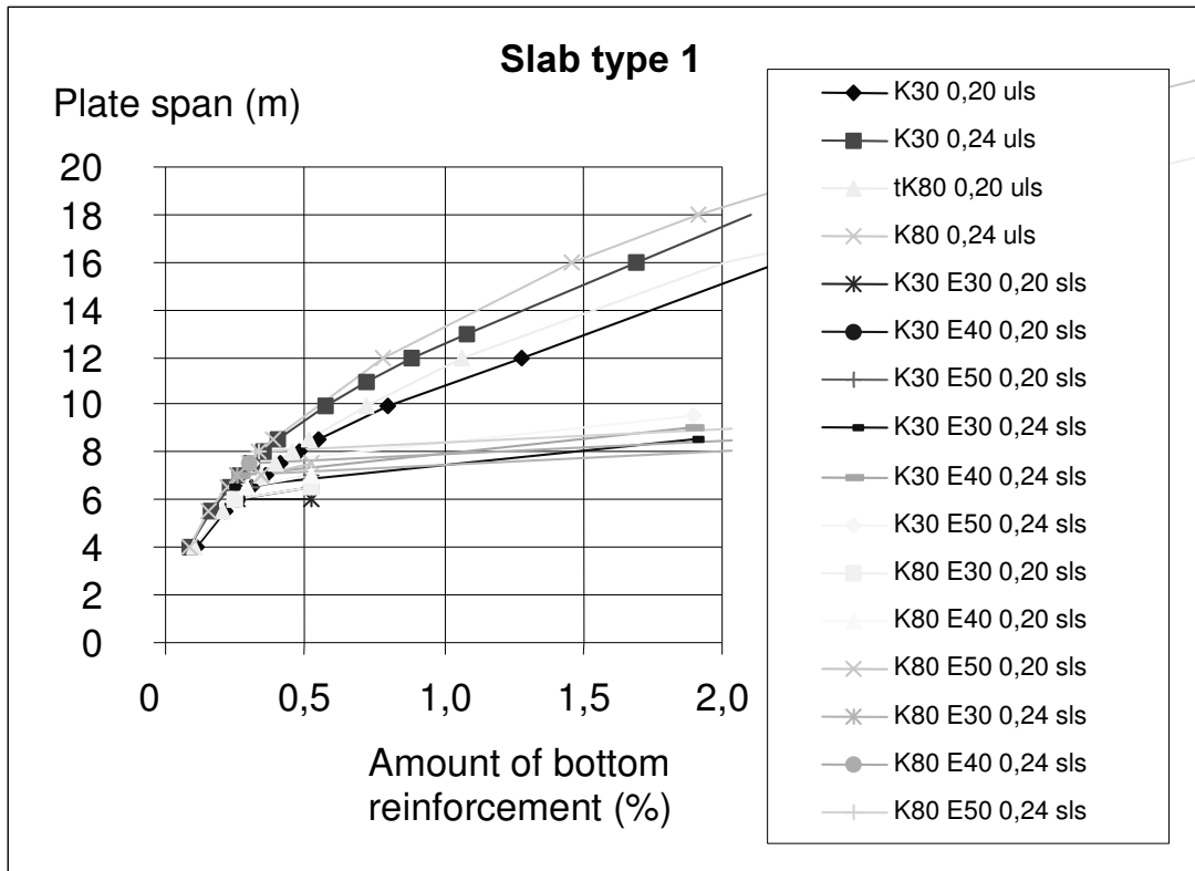
Slab type 1 (Figure 3.2)
