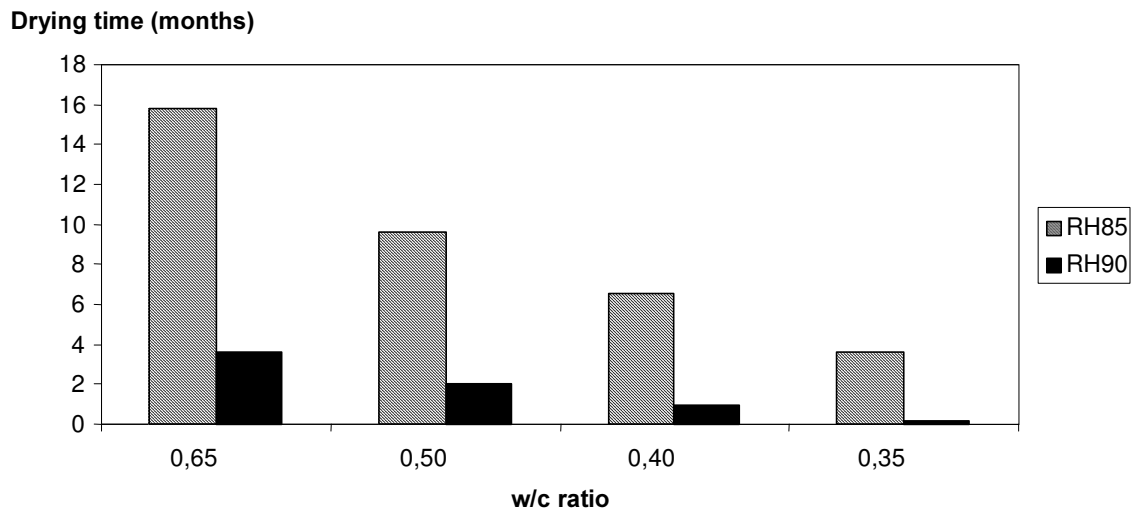
Figure 4.8 Estimated effects of various w/c ratios on the concrete drying time for Climate 2. Constant type of formwork (permanent concrete elements, “Filigran”) and slab thickness (0,20 m) is used within the calculations. No silica fume.
