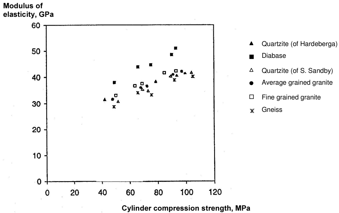
Figure 2.3 Elastic modulus of concrete as function of cylinder compression strength for various qualities of aggregate (Hassanzadeh, 1998).
