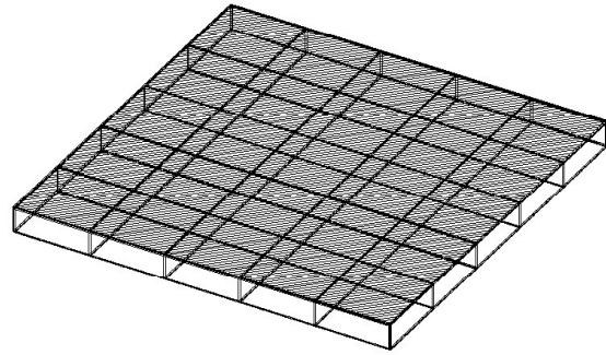
Figure 3.4 Slab type 3, Two-way reinforced inner field.
