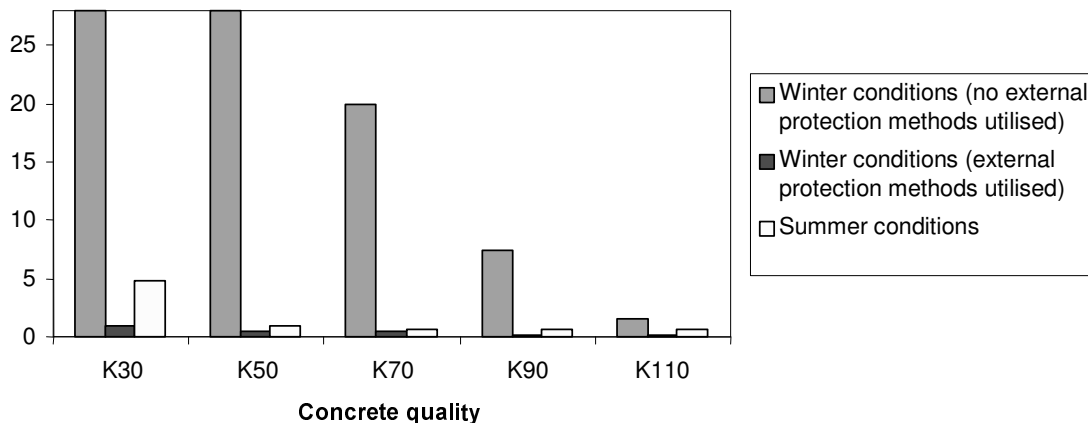
Figure 4.23 Time needed to reach a compressive strength of 20 MPa in a 0,2 m thick member cast in 19 mm Plywood form. Effects of concrete quality and winter precautions are shown. Swedish Standard Portland Cement.
